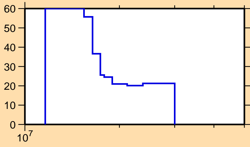
\Delta\sigma/\sigma vs. E for ^{235}\text{U}(\text{mt } 5)
