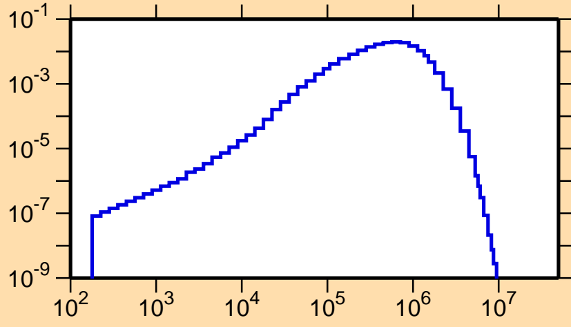
\sigma vs. E for ^{235}\text{U}(n,n_1)
