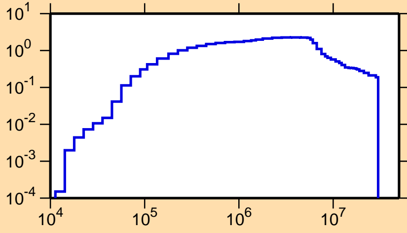
\sigma vs. E for ^{235}\text{U}(\text{mt851})
