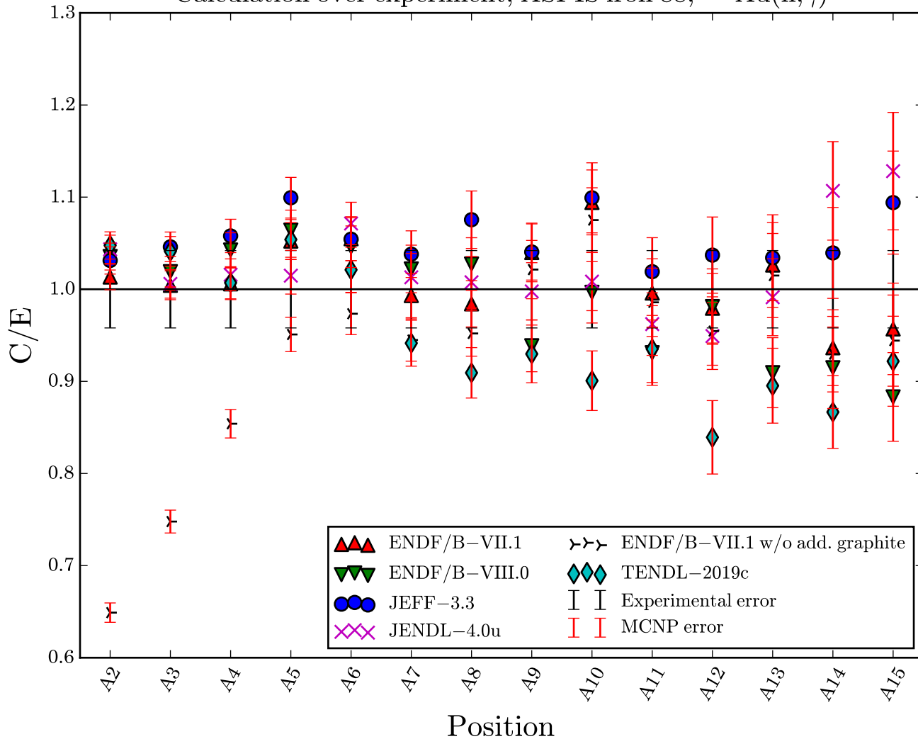
Calculation over experiment, ASPIS iron 88, ^{197}\text{Au}(n,\gamma)
