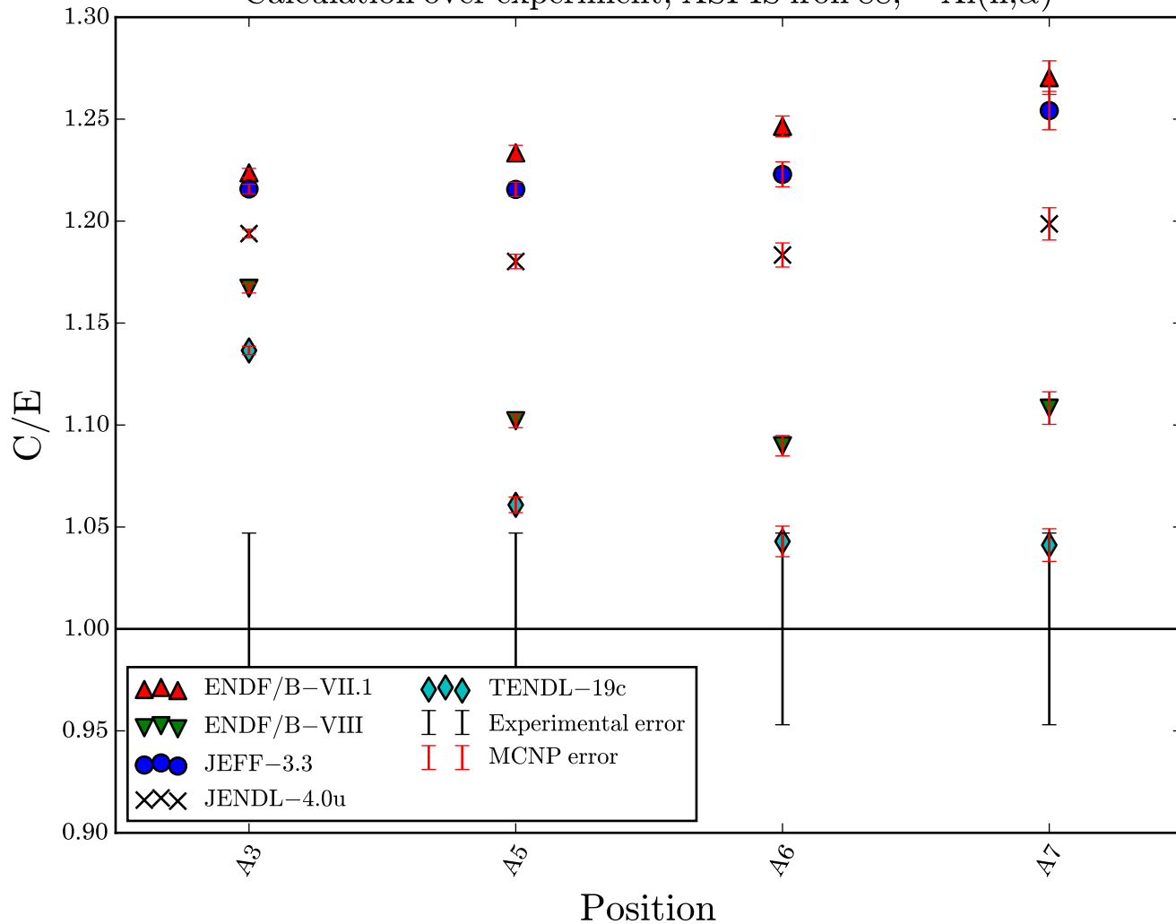
Calculation over experiment, ASPIS iron 88, ^{27}\text{Al}(n,\alpha)
