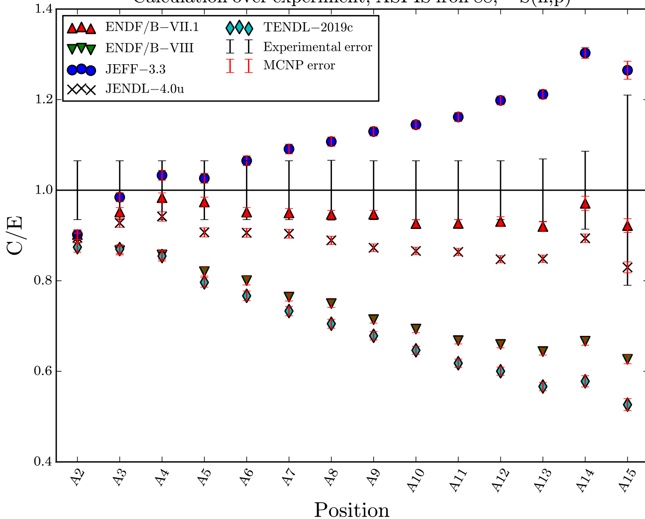
Calculation over experiment, ASPIS iron 88, ^{32}\text{S}(n,p)
