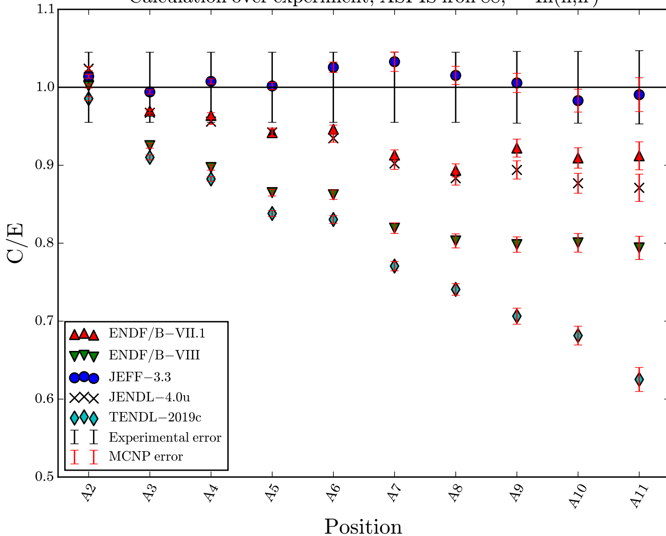
Calculation over experiment, ASPIS iron 88, ^{115}\text{In}(n,n')
