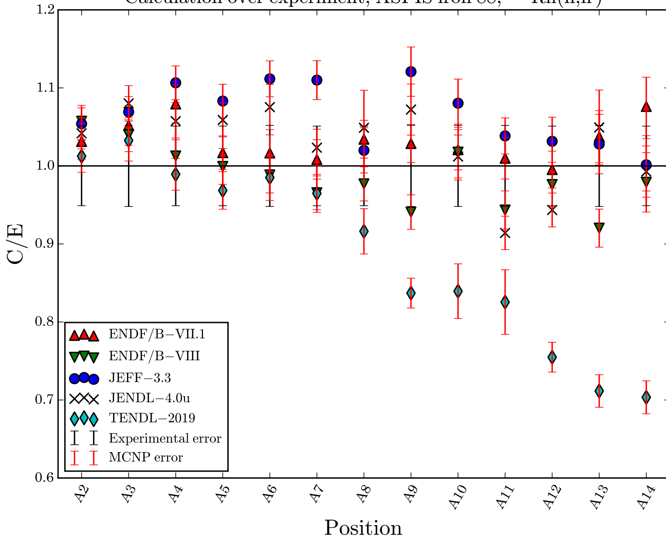
Calculation over experiment, ASPIS iron 88, ^{103}\text{Rh}(n,n')
