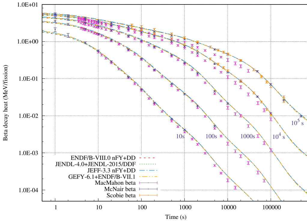
Figure 17: Beta decay heat from 10-100000 s irradiations of 235 U.
