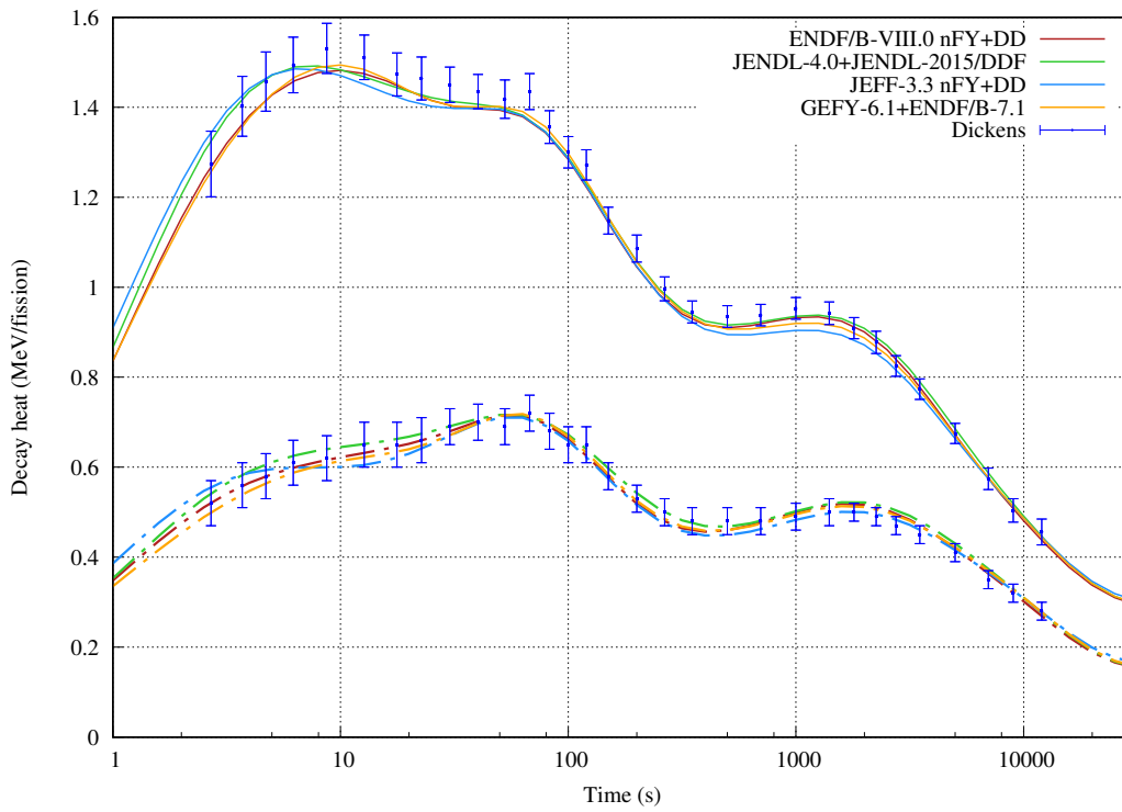
Figure 46: Total (solid) and gamma (dash) decay heat from thermal pulse on ^{241}\text{Pu} .
