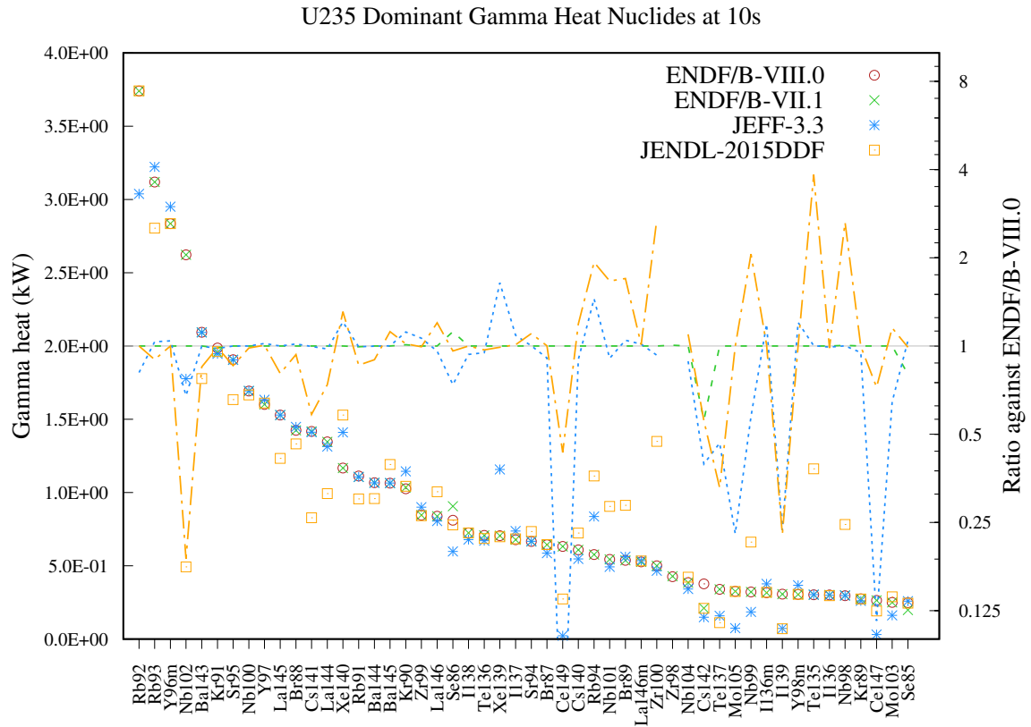
Figure 48: Gamma decay data comparison for U235 fission pulse after 10s cooling.
