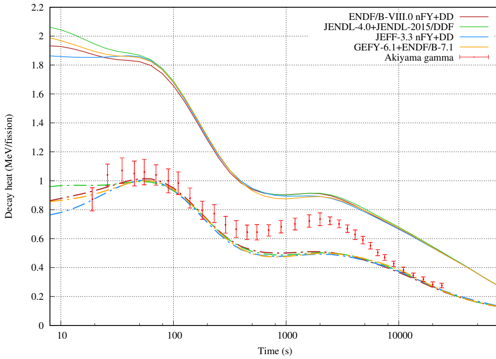
Figure 33: Total (solid) and gamma (dash) decay heat from fast pulse on 232 Th.
