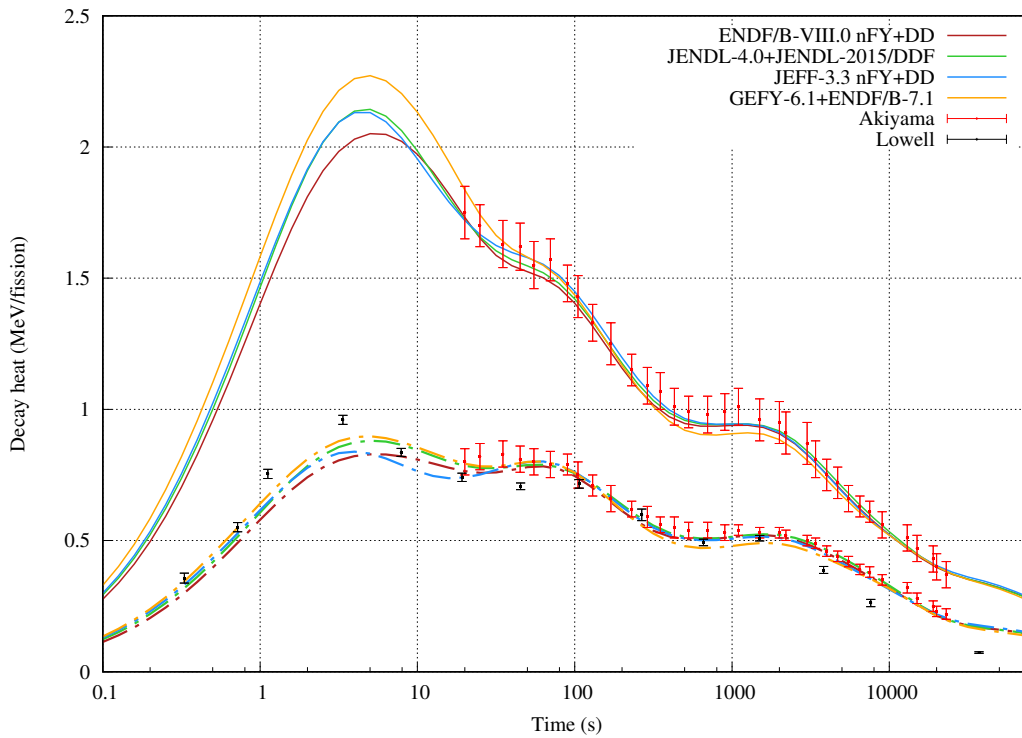
Figure 41: Total (solid) and gamma (dash) decay heat from fast pulse on ^{238}\text{U} .
