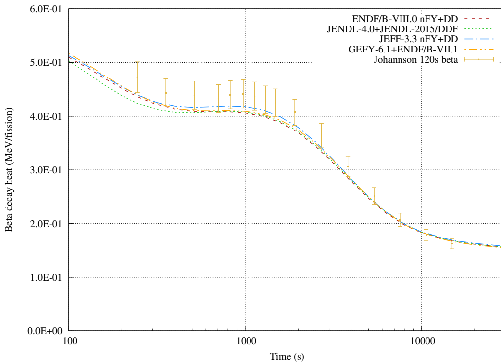
Figure 30: Beta decay heat from 4-120s irradiations of 239 Pu.
