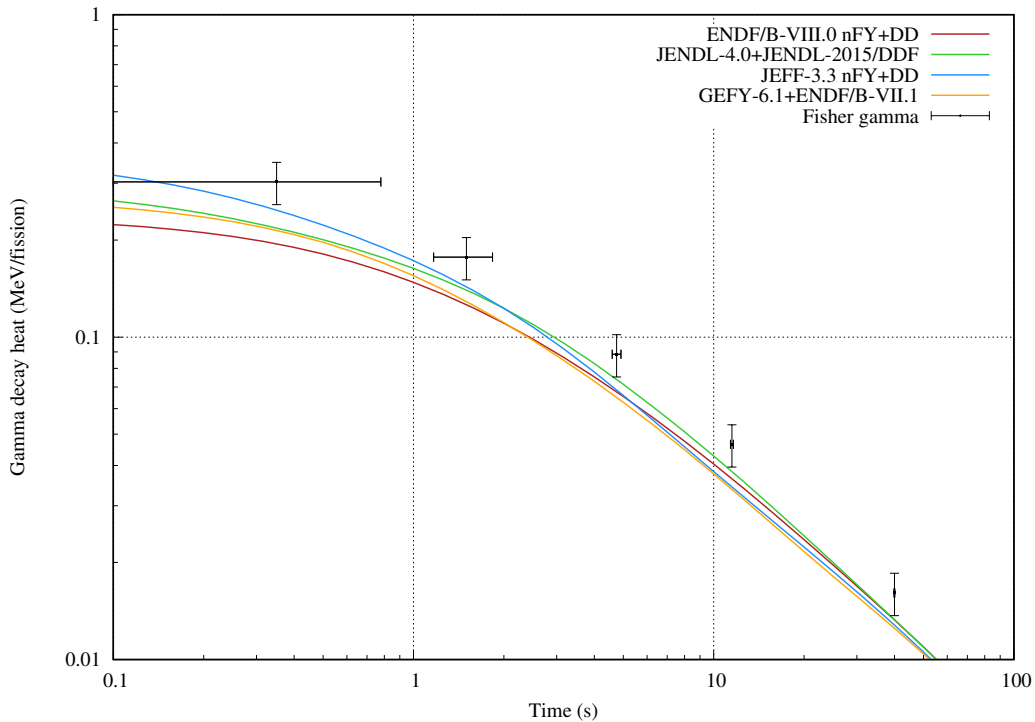
Figure 40: Gamma decay heat from <0.1\text{s} irradiations of ^{233}\text{U} .
