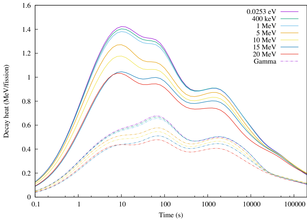
Figure 6: Comparison of total decay heat burst functions of ^{235}\text{U} for various neutron energies. All simulations use GEF-6.1 nFY with ENDF/B-VII.1 decay data.
