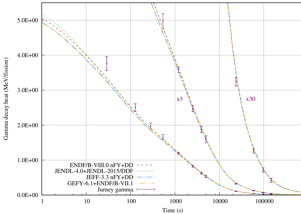
Figure 16: Gamma decay heat from thermal 2E4s irradiation of ^{235}\text{U} .
