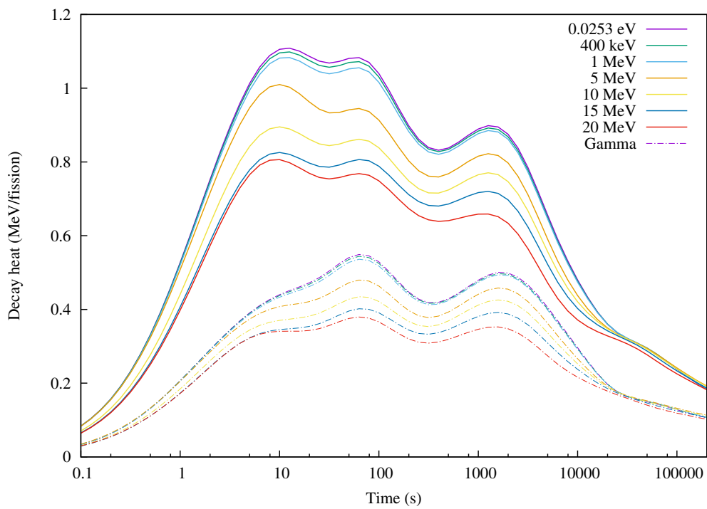
Figure 7: Comparison of total decay heat burst functions of ^{239}\text{Pu} for various neutron energies. All simulations use GEF-6.1 nFY with ENDF/B-VII.1 decay data.
