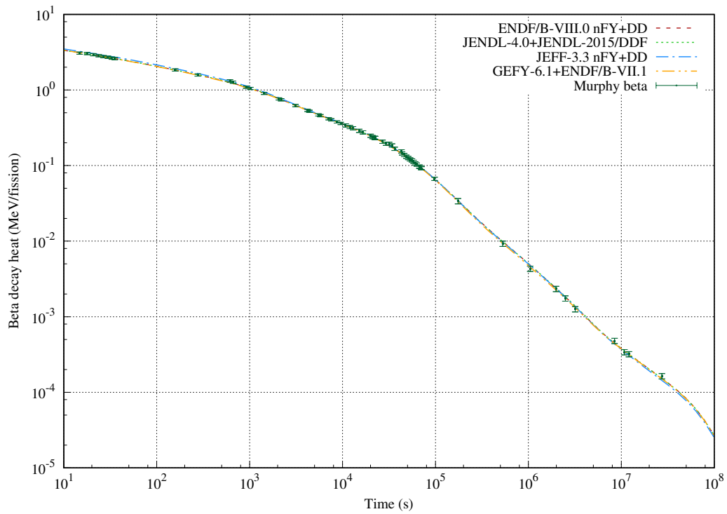
Figure 31: Beta decay heat from 1E5s irradiation of ^{239}\text{Pu} .
