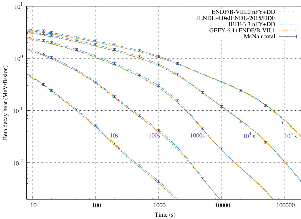
Figure 29: Beta decay heat from 10-100000 s thermal irradiation of 239 Pu.
