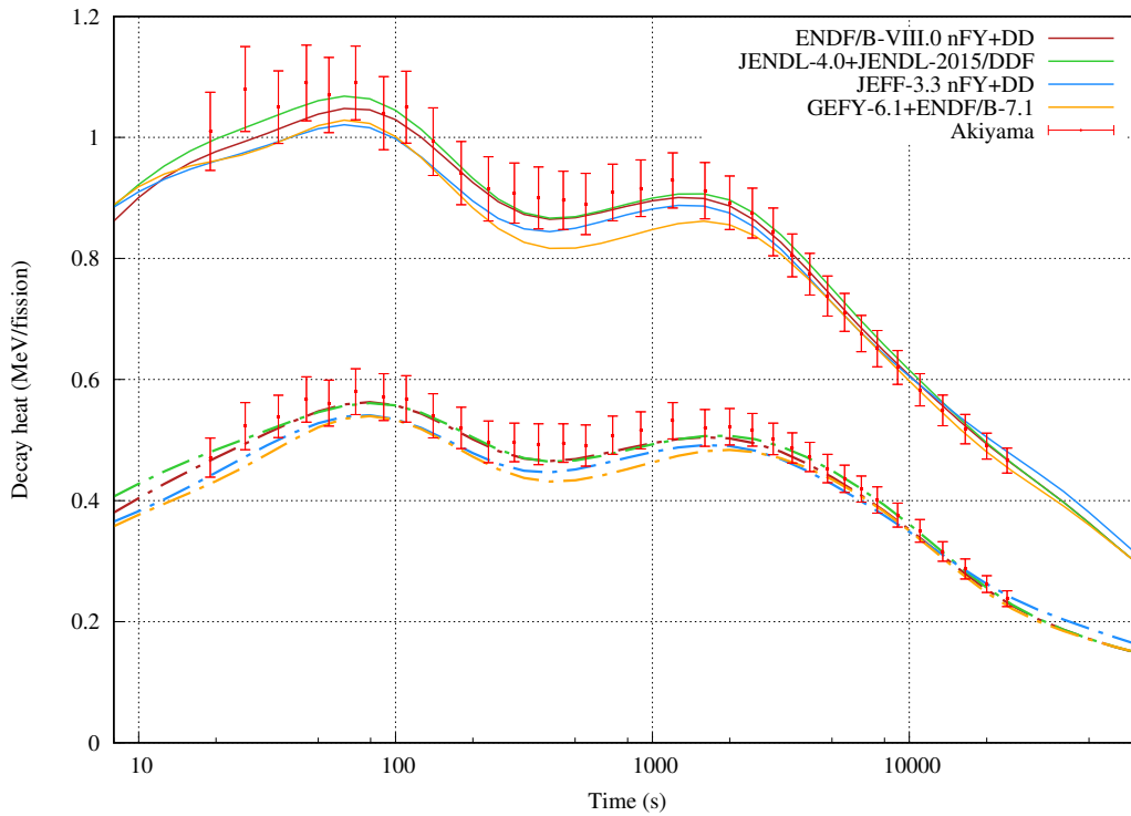
Figure 36: Total (solid) and gamma (dash) decay heat from fast pulse on ^{233}\text{U} .
