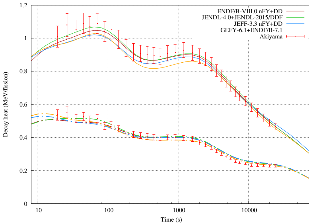
Figure 37: Total (solid) and beta (dash) decay heat from fast pulse on ^{233}\text{U} .
