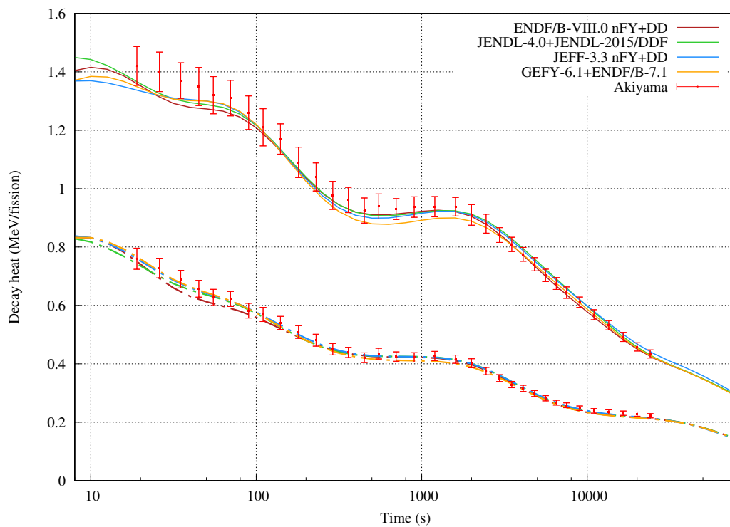
Figure 12: Total (solid) and beta (dash) decay heat from fast pulse on ^{235}\text{U} .
