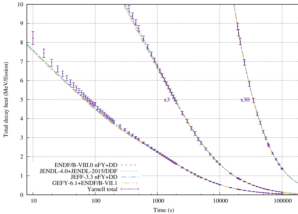
Figure 15: Total decay heat from thermal 2E4s irradiation of ^{235}\text{U} .
