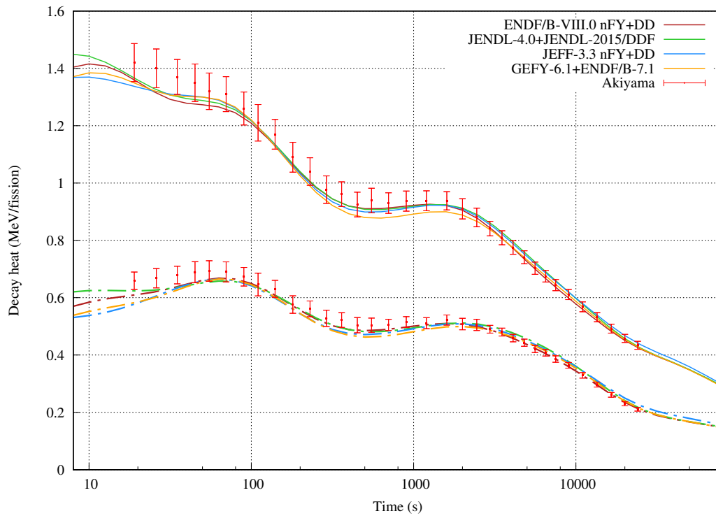
Figure 11: Total (solid) and gamma (dash) decay heat from fast pulse on ^{235}\text{U} .
