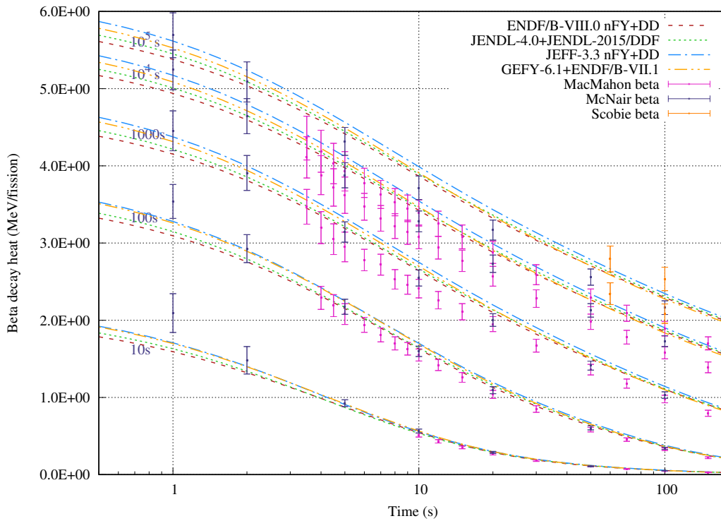
Figure 18: Beta decay heat from 10-100000 s irradiations of 235 U for <200 s cooling.
