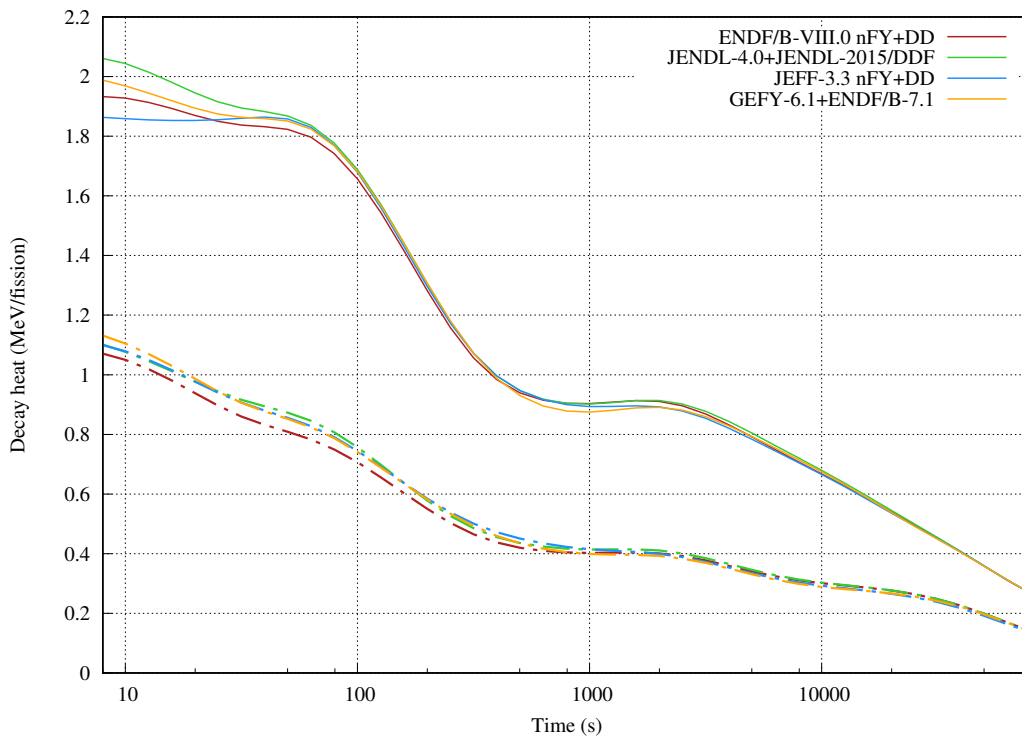
Figure 34: Total (solid) and beta (dash) decay heat from fast pulse on 232 Th.
