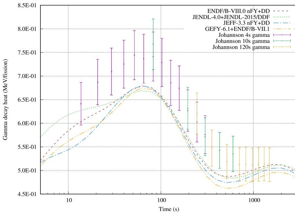
Figure 22: Gamma decay heat from 4-120s irradiations of ^{235}\text{U} .
