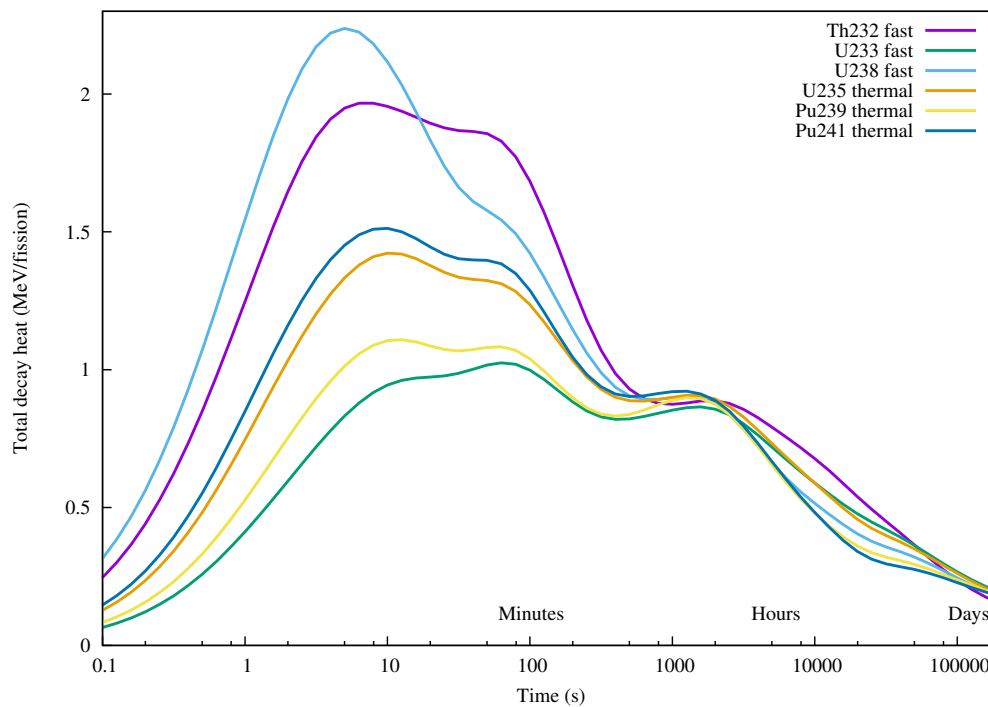
Figure 5: Comparison of total decay heat burst functions for various nuclides of interest for reactor operation. All simulations use GEF-6.1 nFY with ENDF/B-VII.1 decay data.
