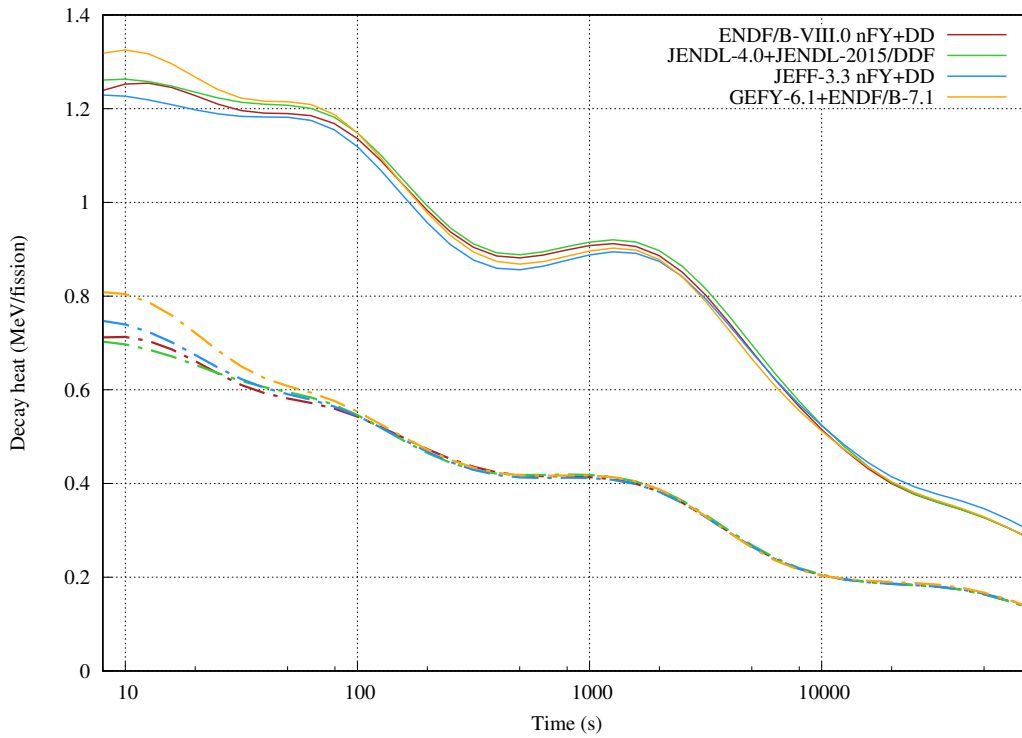
Figure 45: Total (solid) and beta (dash) decay heat from fast pulse on 237 Np.
