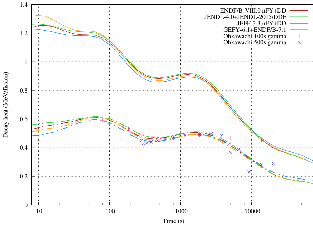
Figure 44: Total (solid) and gamma (dash) decay heat from fast pulse on 237 Np.
