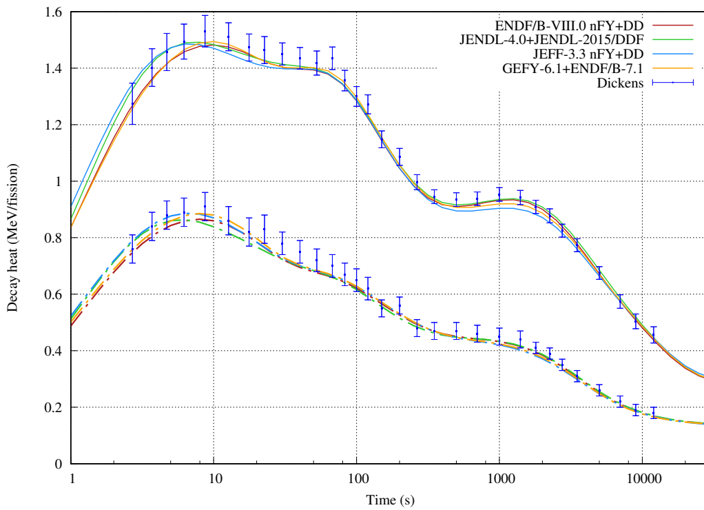
Figure 47: Total (solid) and beta (dash) decay heat from thermal pulse on ^{241}\text{Pu} .
