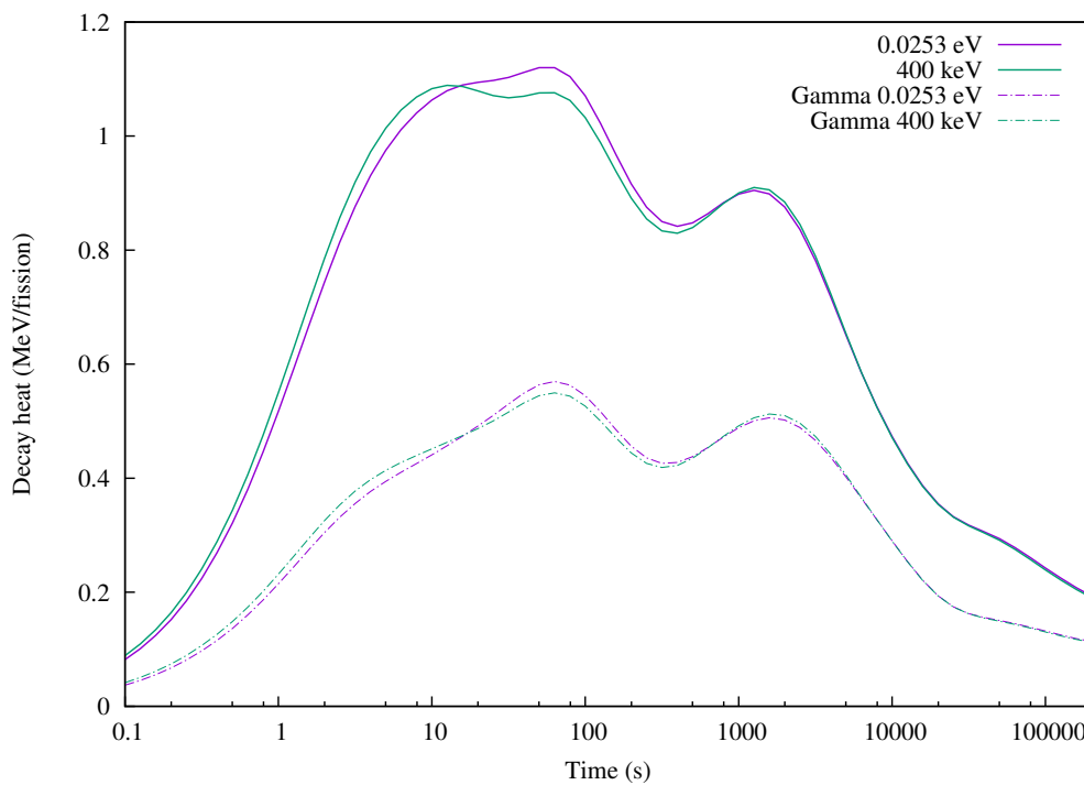
Figure 8: Comparison of total decay heat burst functions of ^{239}\text{Pu} for all energies within the JEFF-3.3 nFY file.
