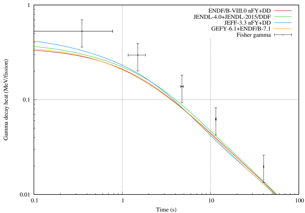
Figure 32: Gamma decay heat from <0.1\text{s} irradiations of ^{239}\text{Pu} .
