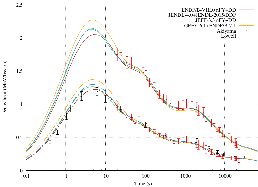
Figure 42: Total (solid) and beta (dash) decay heat from fast pulse on ^{238}\text{U} .
