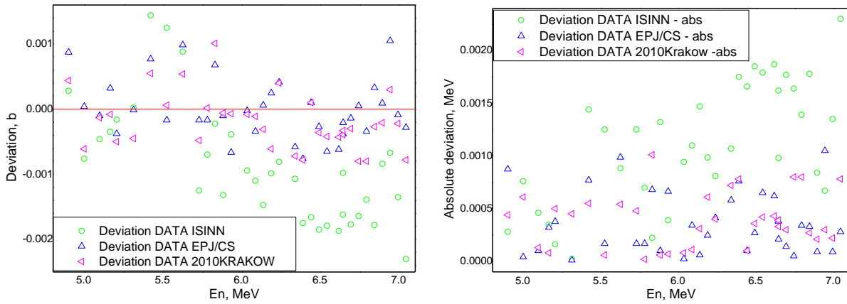
FIG. 4 (colour online). Deviation (left) and absolute deviation (right) of digitized DATA values from author’s data.
